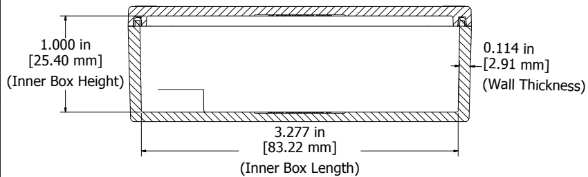
SECTION E-E Side View of Assembly
