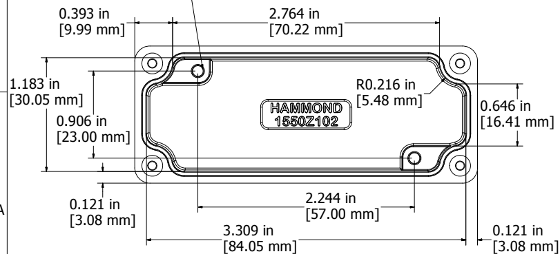
Top View Looking Inside Box
