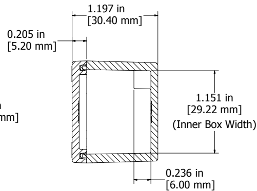
SECTION F-F End View of Assembly
