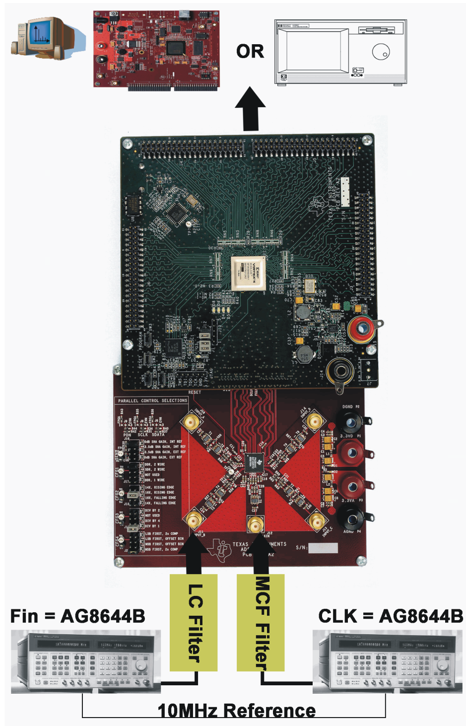
Figure 3. ADS62xxEVM Setup
