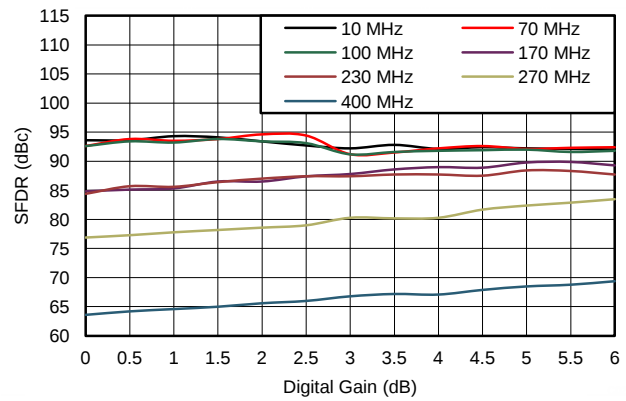
Figure 53. SFDR vs Digital Gain and Input Frequency
