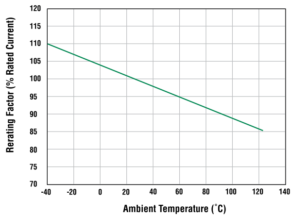
MAXI Fuse Temperature Derating Curve
