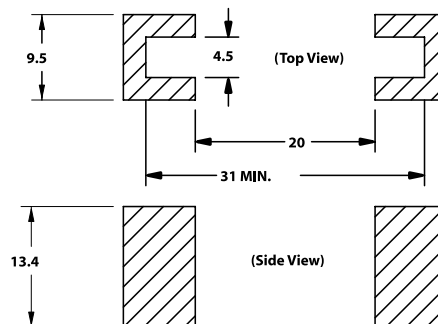
Recommended Mating Cavity
