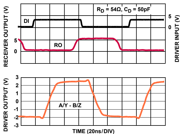
FIGURE 27. DRIVER AND RECEIVER WAVEFORMS (ISL31478E)
