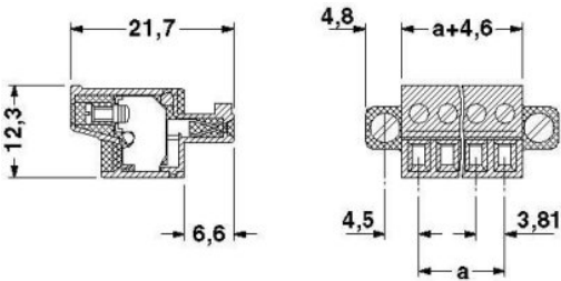
Dimensioned drawing
