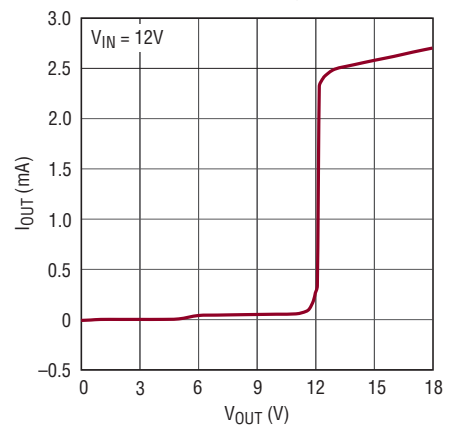
OUT Current vs Voltage
