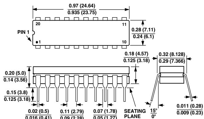
20-Lead Cerdip (Q-20)
