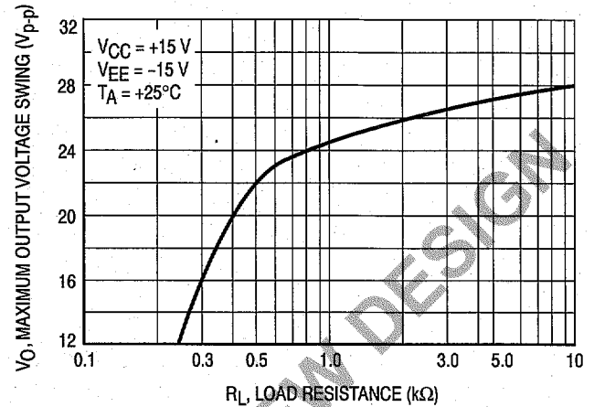
Figure 2. Maximum Output Voltage Swing versus Load Resistance
