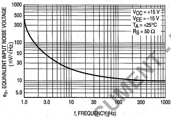
Figure 3. Equivalent Input Noise Voltage versus Frequency
