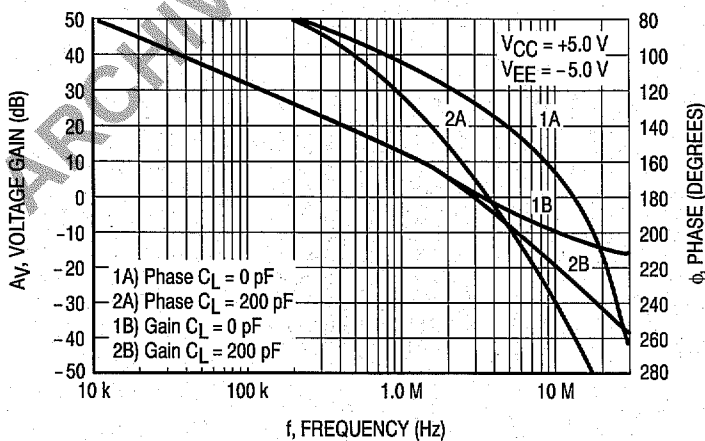
Figure 5. Voltage Gain and Phase versus Frequency
