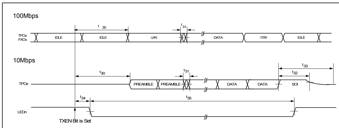
FIGURE 36 - TRANSMIT TIMING
