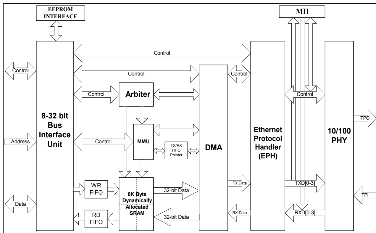
FIGURE 4 - BLOCK DIAGRAM
