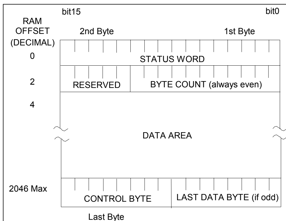
FIGURE 14 - DATA FRAME FORMAT
