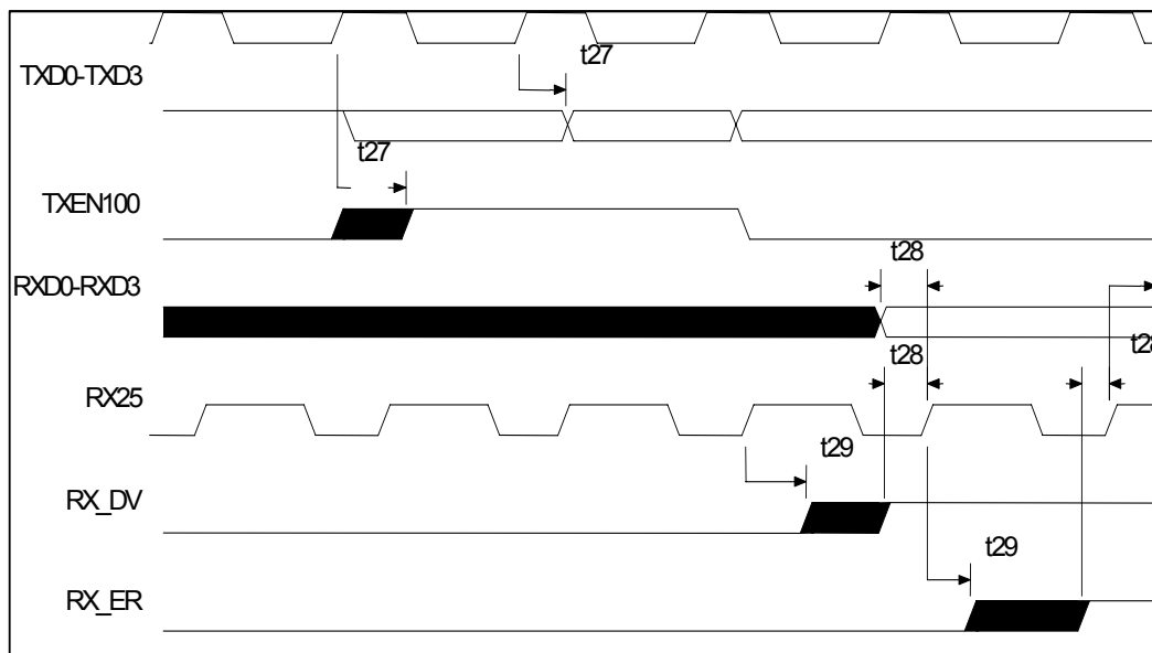
FIGURE 35 - MII TIMING
