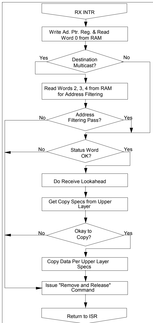
FIGURE 17 - RX INTR
