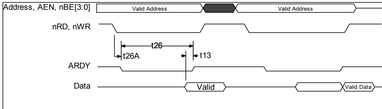
FIGURE 29 - ASYNCHRONOUS READY
