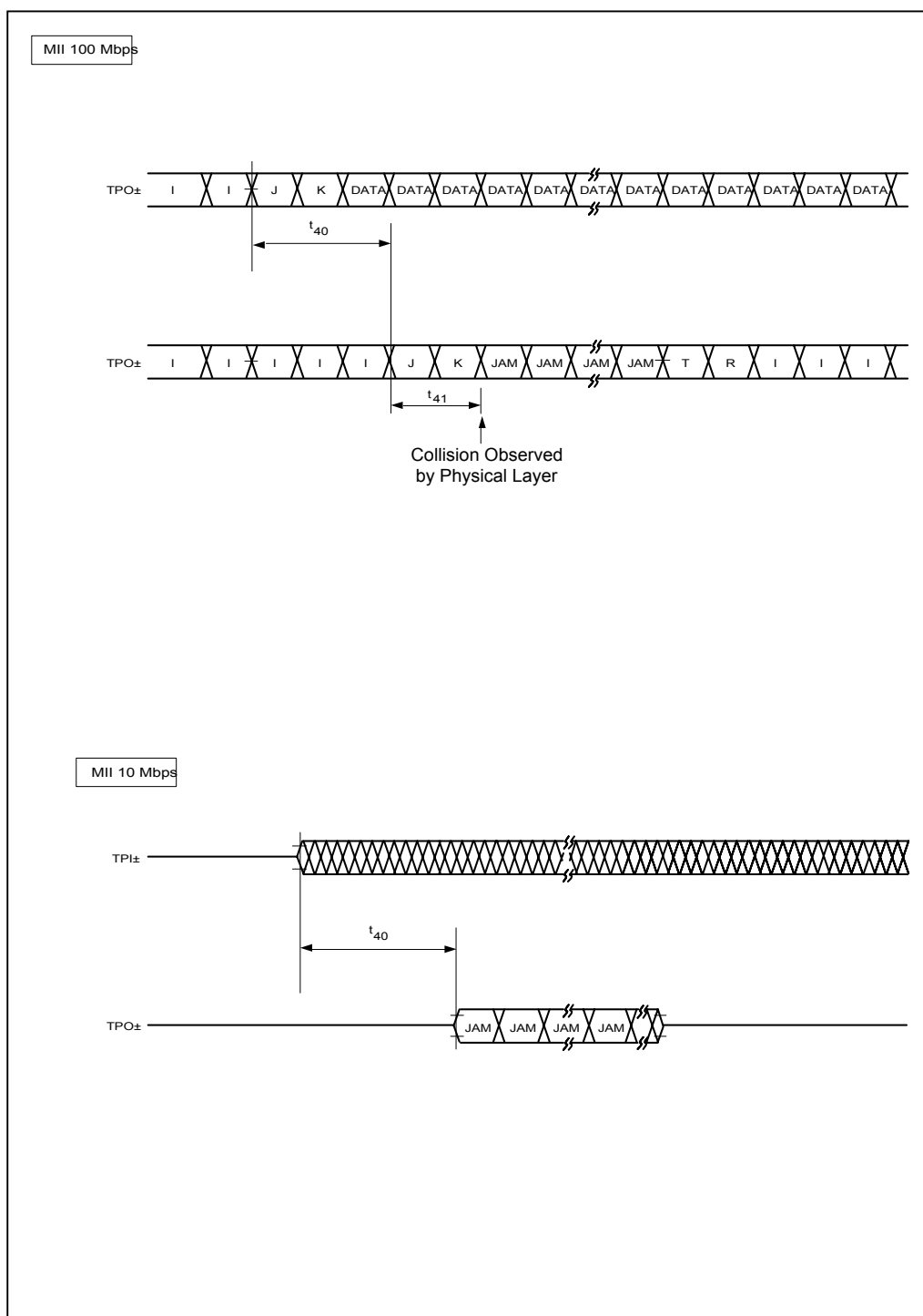
FIGURE 40 - JAM TIMING
