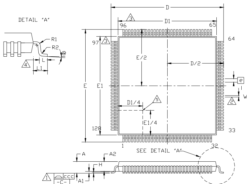
FIGURE 43 - 128 PIN TQFP, 14X14X1.0 BODY
