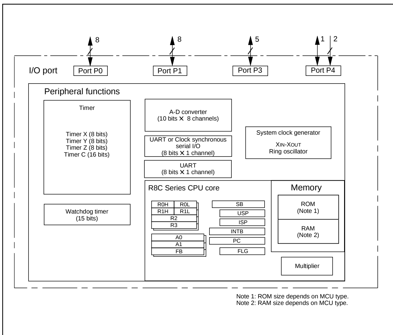
Figure 1.1 Block Diagram
