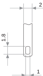
Switch terminal detail.
