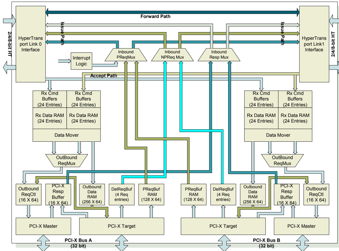
Figure 2: Block Diagram
