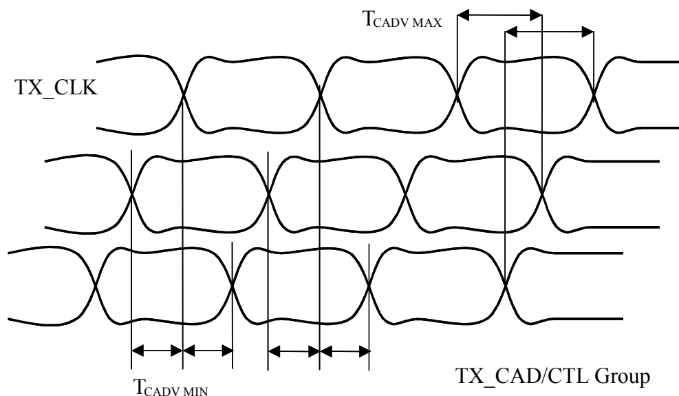
Figure 12: T_{CADV}
