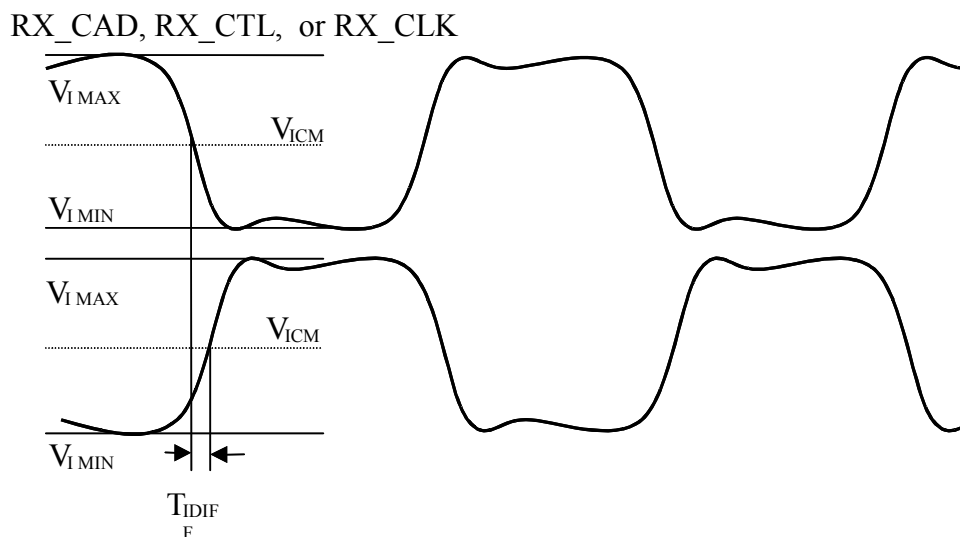
Figure 13: T_{IDIFF}
