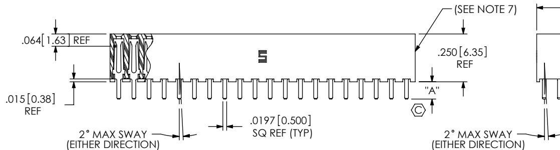
FIG 1 SQT-120-0T-XX-6 SHOWN
