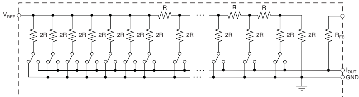
Figure 38. Equivalent R-2R DAC Circuit
