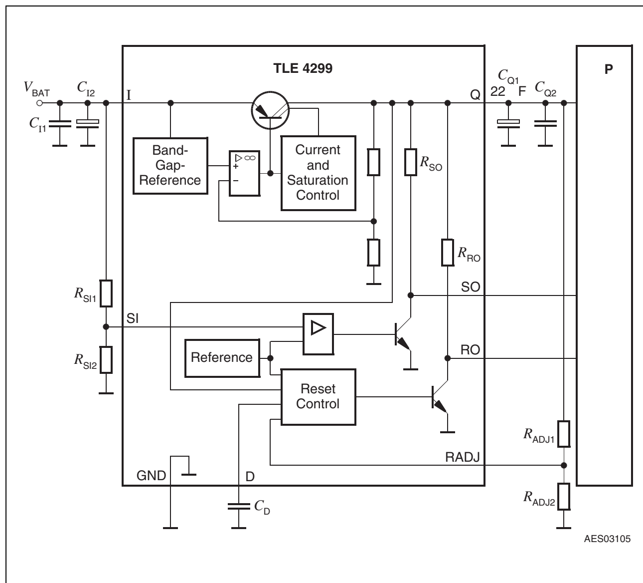
Figure 6 Application Diagram TLE 4299 GV33
