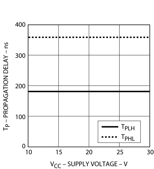
Figure 8 Propagation Delay vs. V_{CC}
