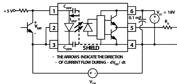
Figure 21 Equivalent Circuit for Figure 15 During CM Transient
