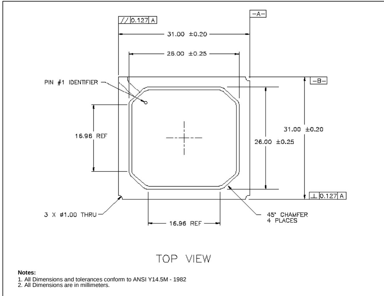
Figure 4. Intel® 82801E C-ICH Package (Top View)
