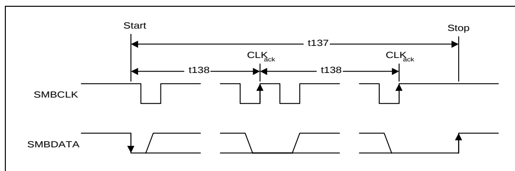
Figure 25. SMBus Time-out
