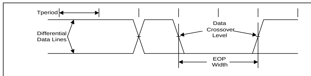
Figure 24. SMBus Transaction
