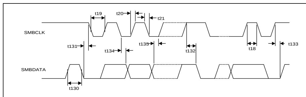
Figure 25. SMBus Time-out
