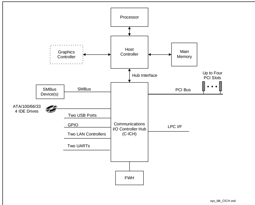
Figure 1. System Configuration
