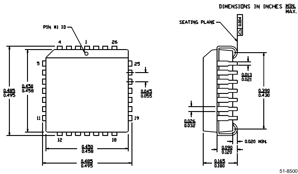
28-lead Plastic Leaded Chip Carrier J64
