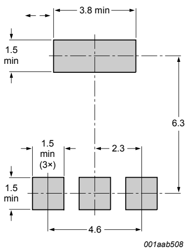
Fig. 8. Minimum footprint SOT223
