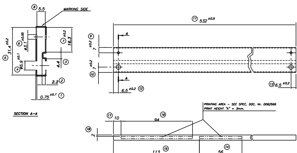
Figure 40. Tube for TO-220 (dual gauge) (mm.)
