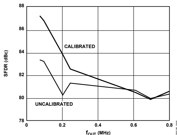
Figure 86. AD9707 SFDR vs. f_{OUT} at 175 MSPS and I_{OUTFS} = 2\text{ mA}
