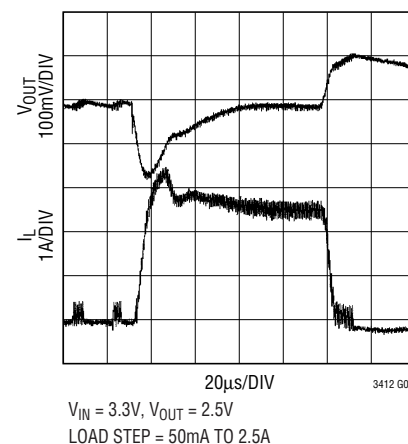
Load Step Transient Burst Mode Operation
