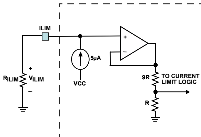
FIGURE 74. CURRENT LIMIT BLOCK DIAGRAM
