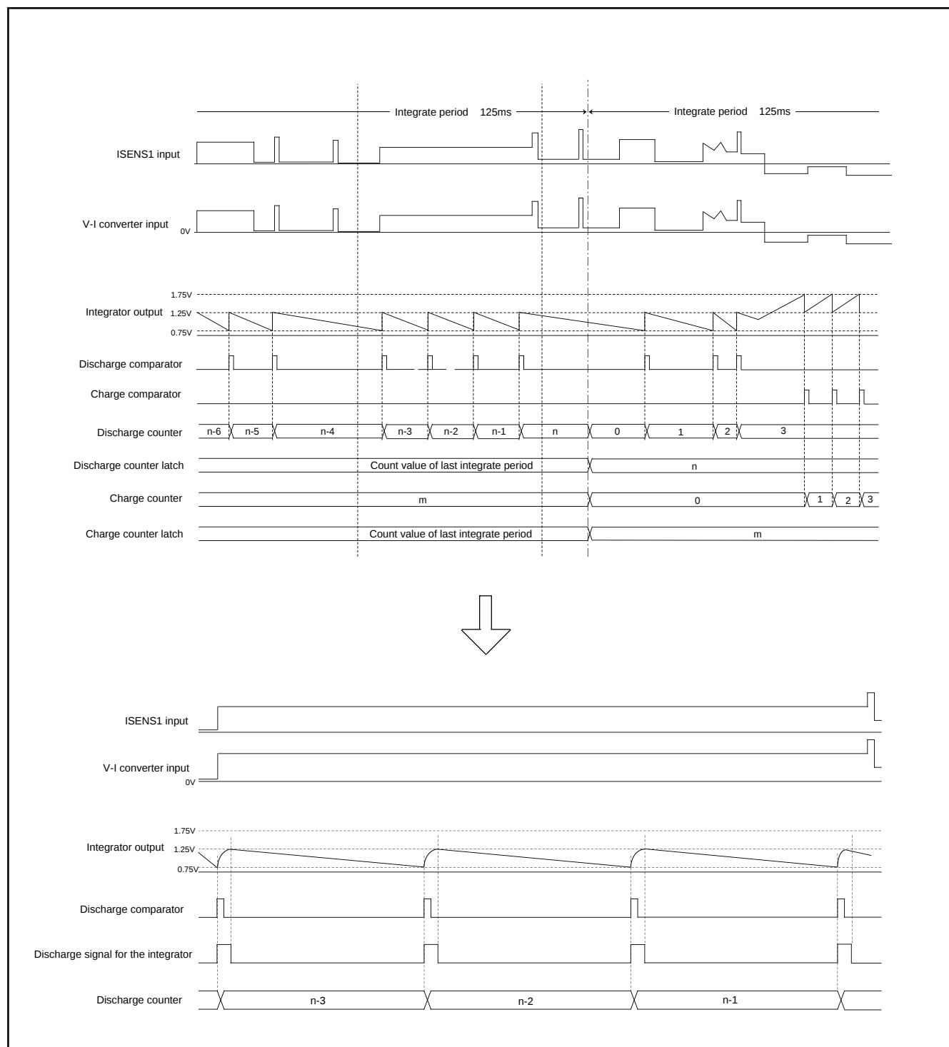
Fig. 48 Current integrator timing diagram
