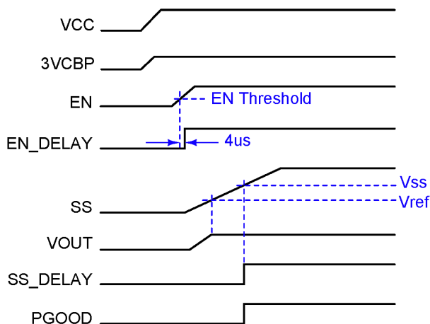
Figure 23: Normal Startup
