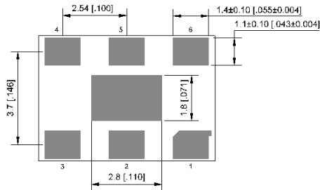
External Dimensions
