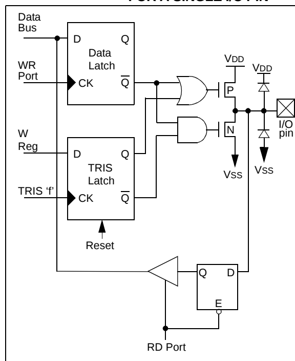
FIGURE 6-1: EQUIVALENT CIRCUIT FOR A SINGLE I/O PIN
