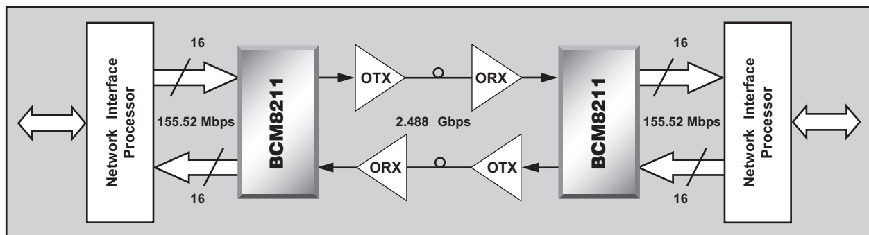
BCM8211 Application Block Diagram
