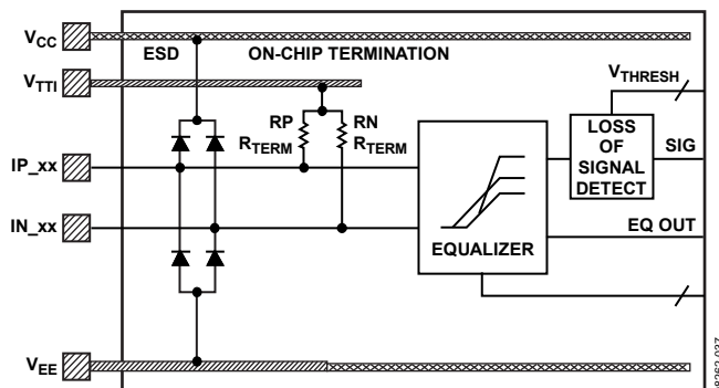
Figure 38. Functional Diagram of the AD8155 Receiver
