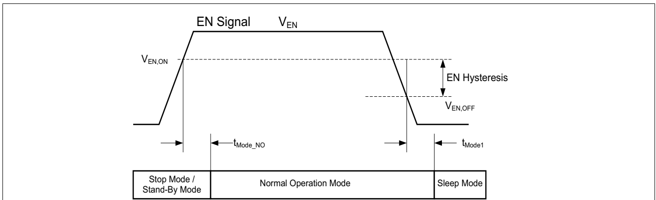
Figure 8 Mode Transition via EN pin
