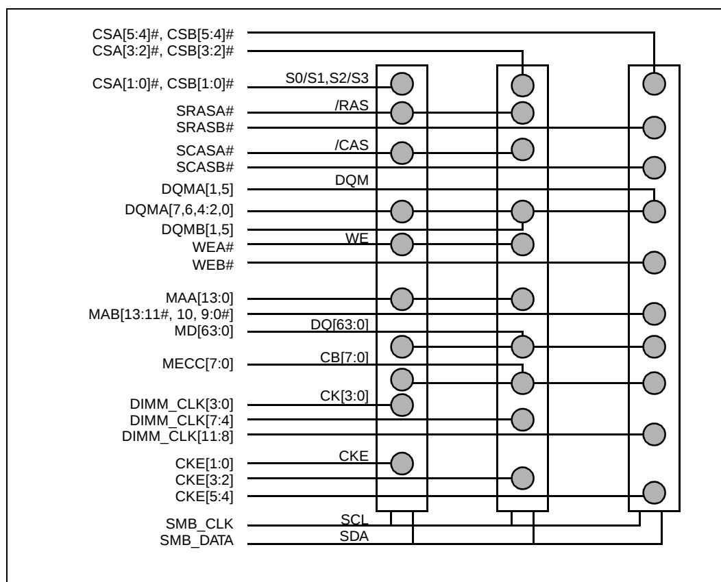
Figure 4-3. Three-DIMM SDRAM Configuration
