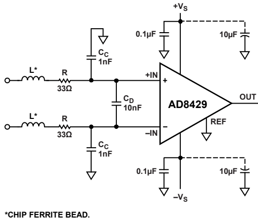
Figure 53. RFI Suppression
