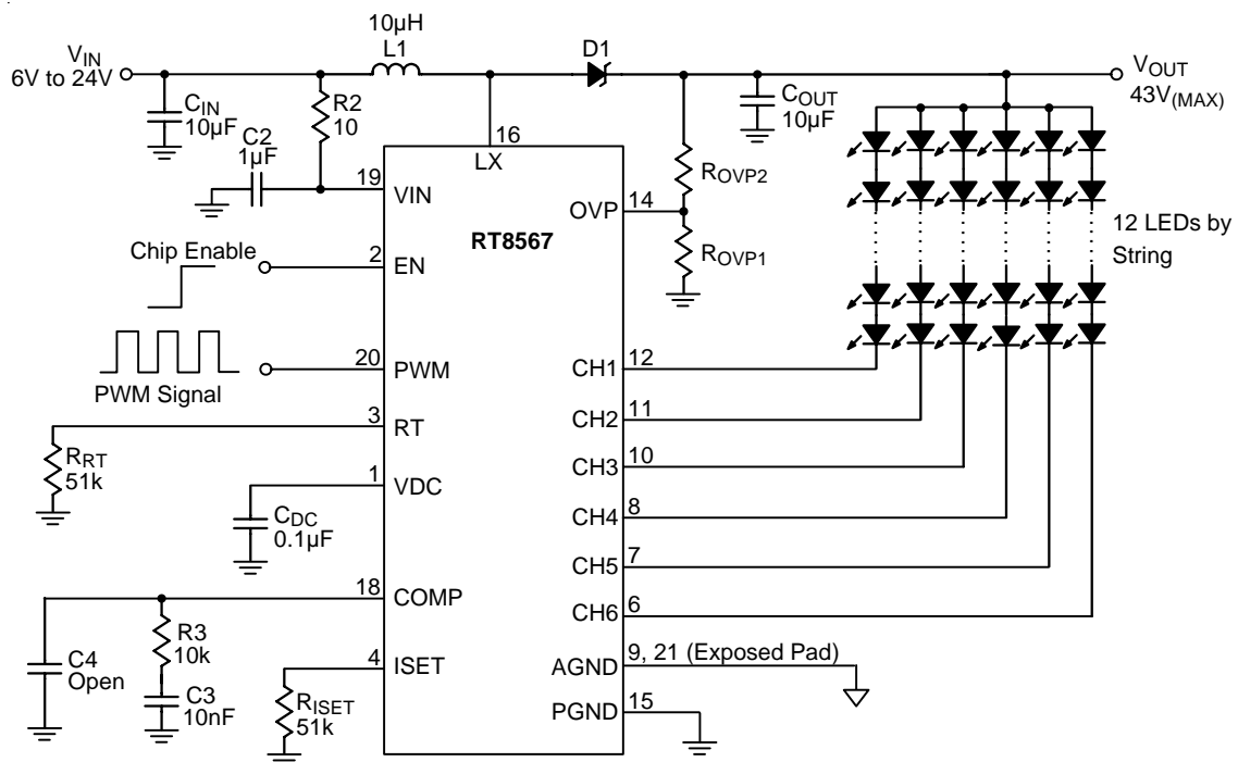
Figure 2. Application Circuit 2
