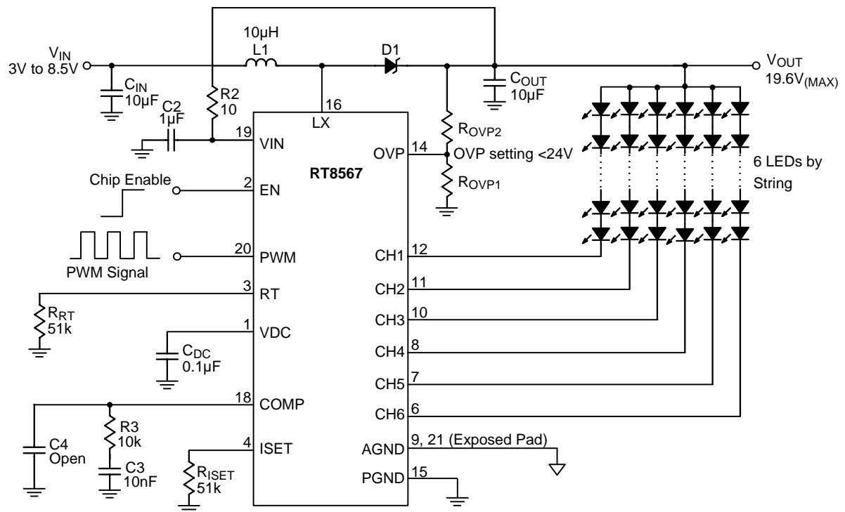
Figure 1. Application Circuit 1
