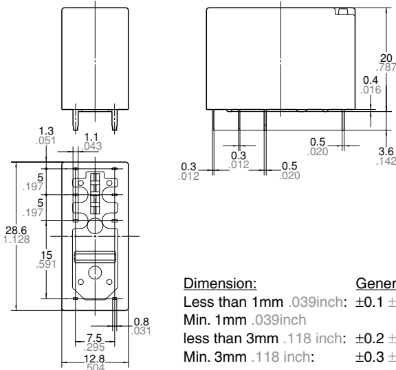
External dimensions
