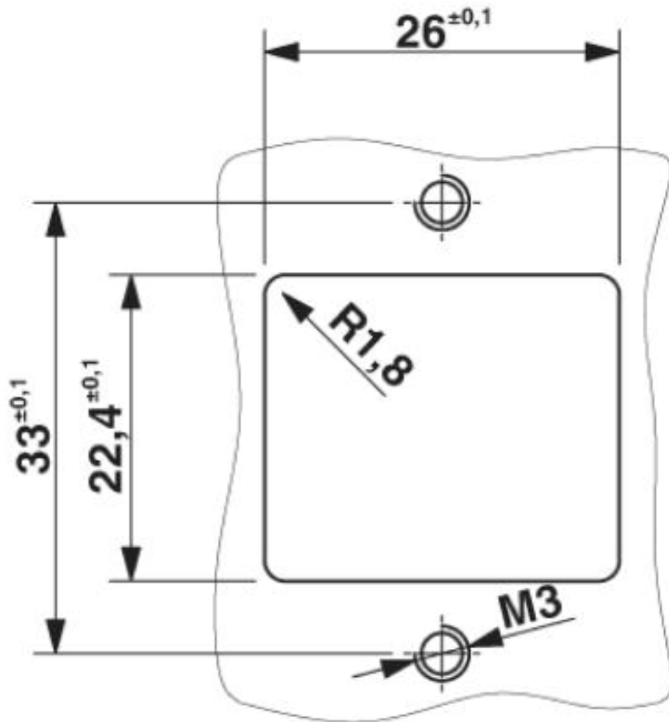
Dimensional drawing
