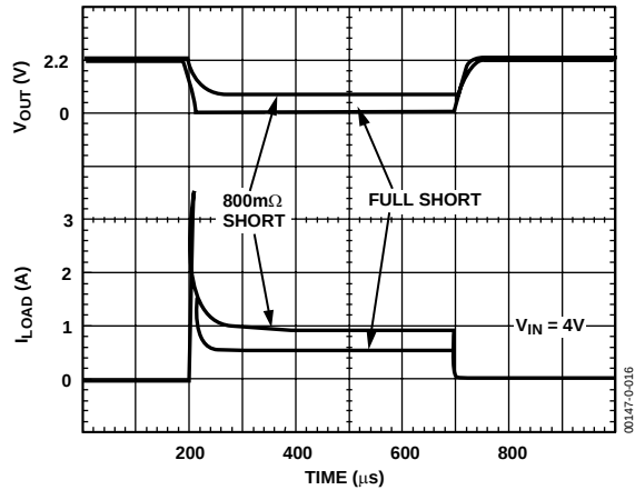
Figure 18. Short-Circuit Current
