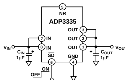
Figure 2. Typical Application Circuit
