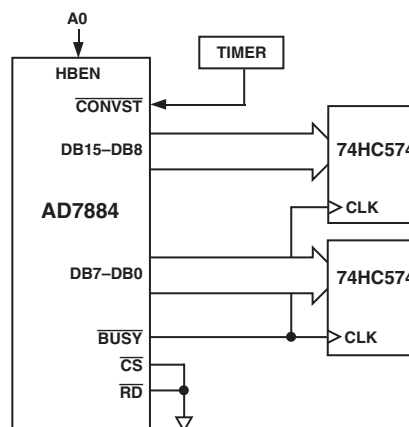
Figure 22. Stand-Alone Operation
