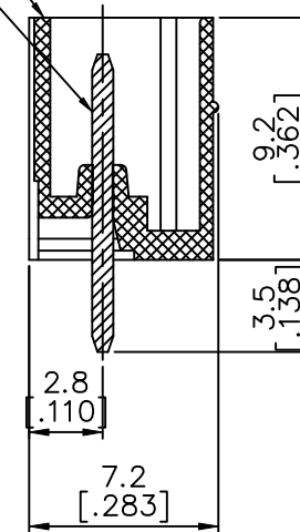
SECTION P-P
