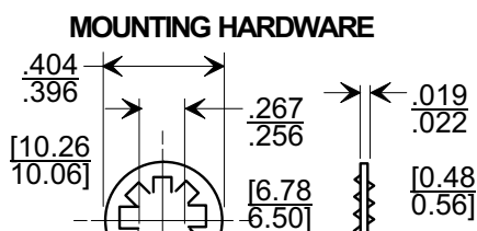
LOCK WASHER
