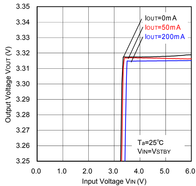
Figure 15. Line Regulation
