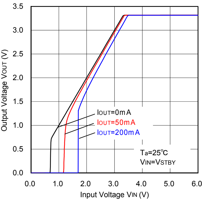
Figure 14. Output Voltage vs. Input Voltage
