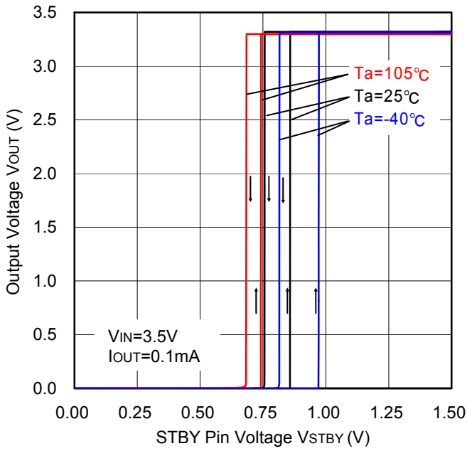
Figure 22. STBY Threshold
