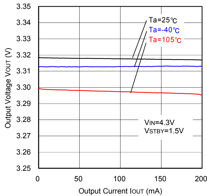
Figure 17. Load Regulation
