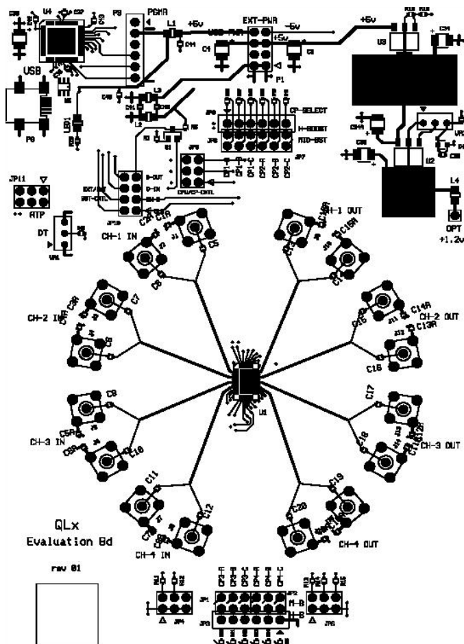
FIGURE 1. QLx4600-S30 EVALUATION BOARD PCB
