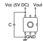
Terminal connection diagram
