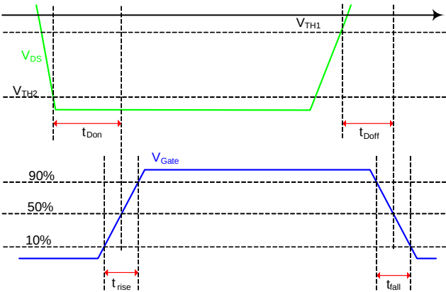
Figure 4: Timing waveform
