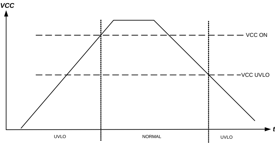
Figure 3: Vcc UVLO
