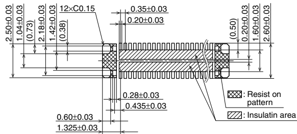
Recommended PC board pattern (TOP VIEW)
