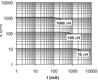
Typical L vs Current
