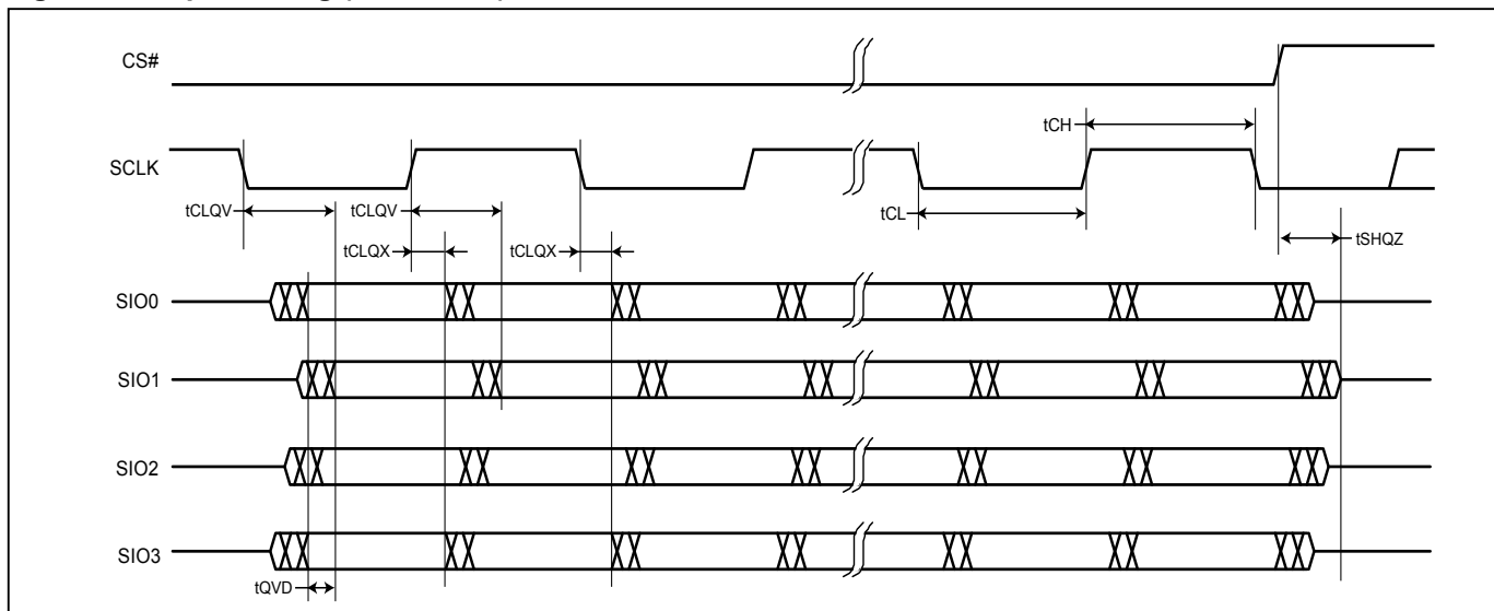
Figure 4. Output Timing (DTR mode)
