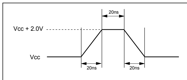
Figure 90. Maximum Positive Overshoot Waveform
