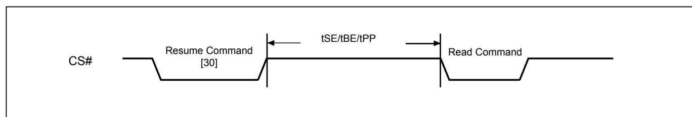
Figure 82. Resume to Read Latency
