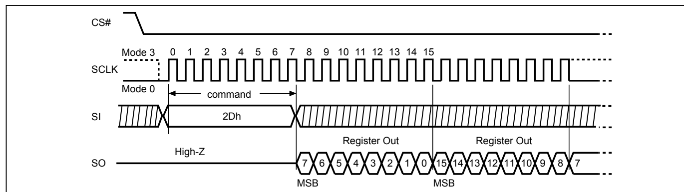
Figure 74. Read Lock Register (RDLR) Sequence
