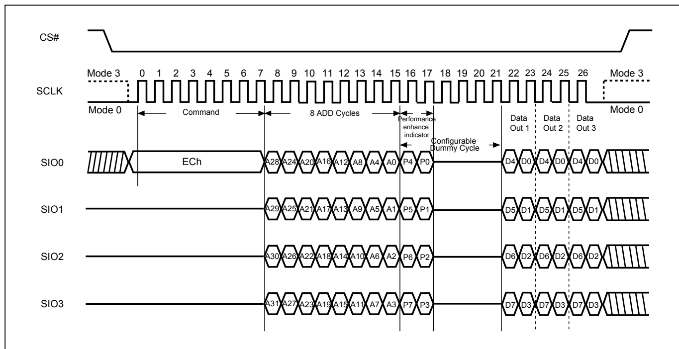
Figure 48. 4 I/O Fast Read using 4 Byte Address sequence (4READ4B)
