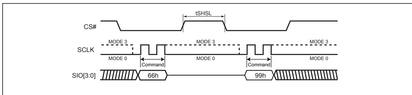
Figure 86. Reset Sequence (QPI mode)
