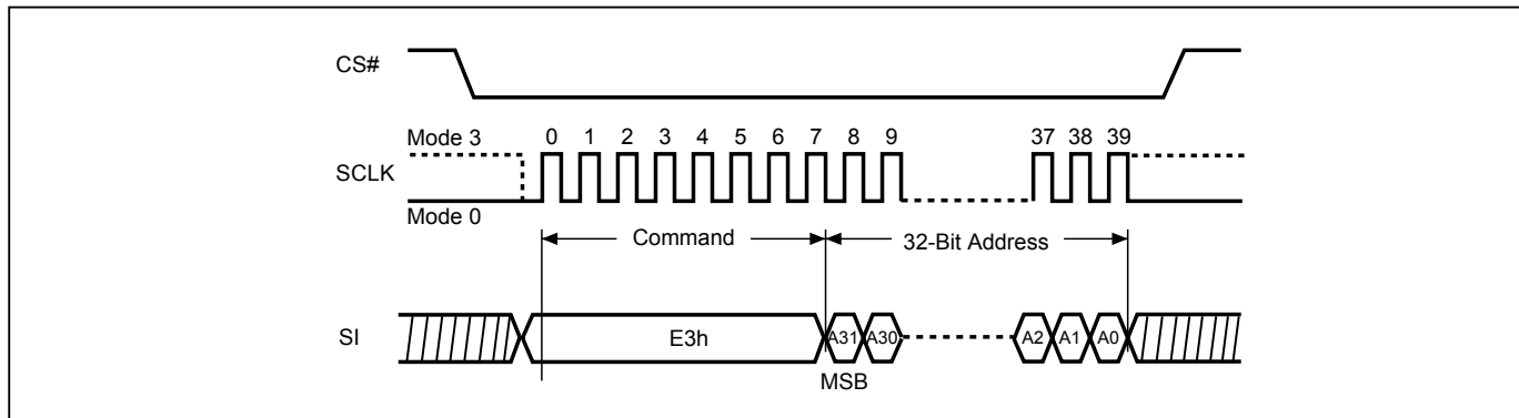
Figure 78. SPB Program (WRSPB) Sequence
