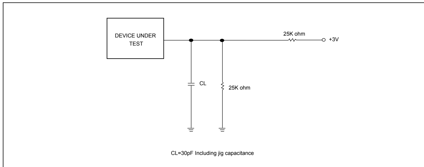
Figure 92. OUTPUT LOADING
