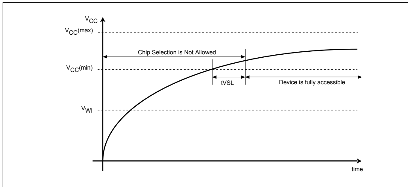
Figure 96. Power-up Timing
