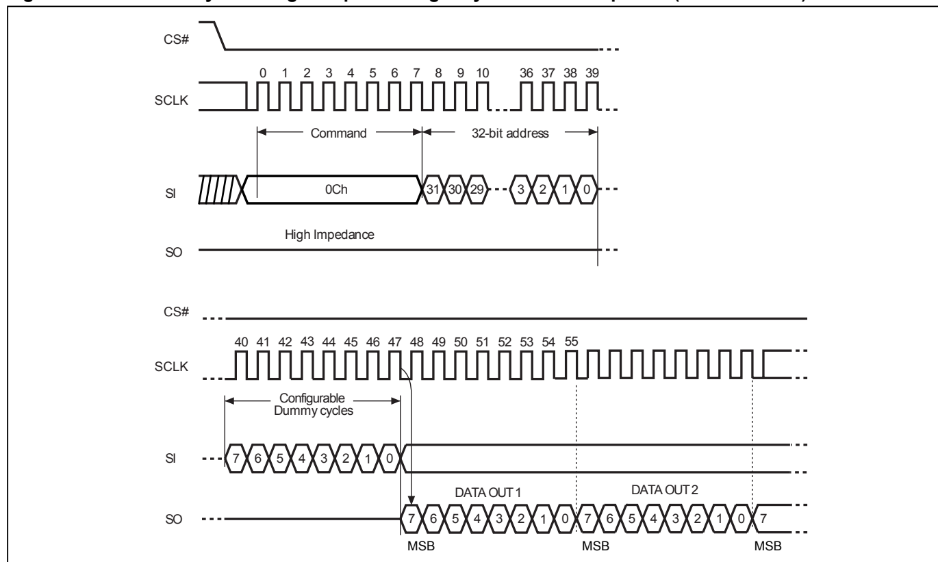
Figure 46. Read Data Bytes at Higher Speed using 4 Byte Address Sequence (FASTREAD4B)
