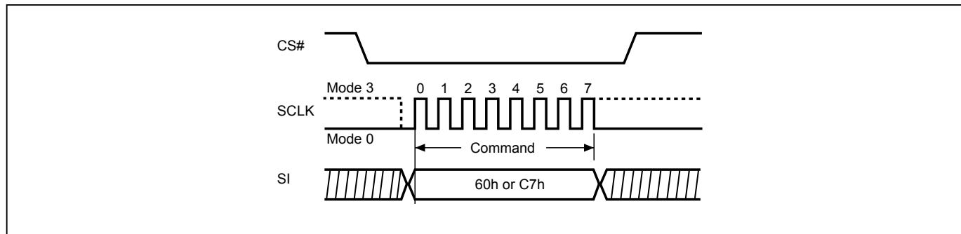
Figure 61. Chip Erase (CE) Sequence (SPI Mode)
