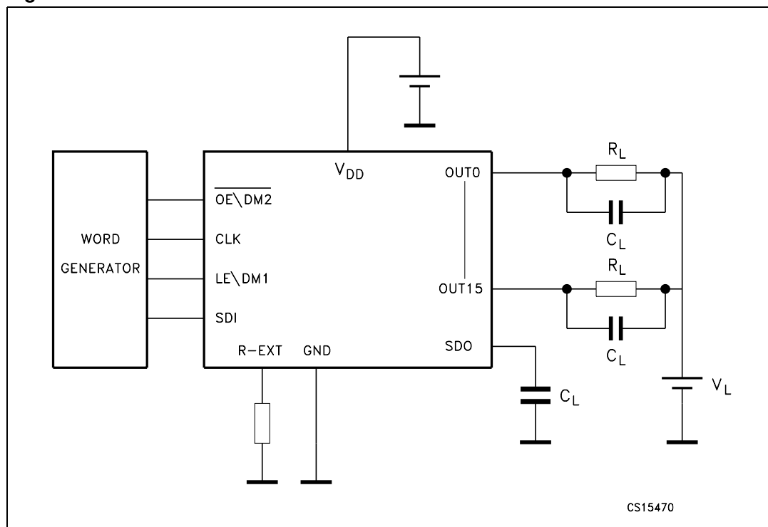
Figure 14. AC characteristics
