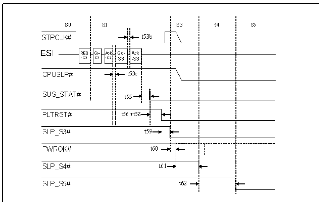
Figure 10-3. ICH Timing Diagram for S4,S5 Transition
