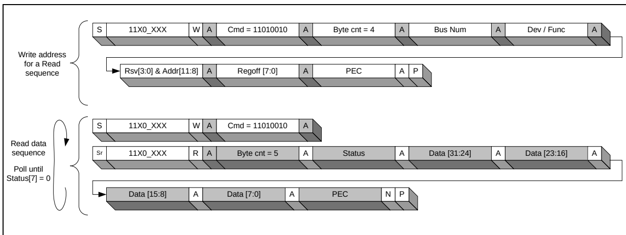
Figure 3-2. SMBus Block-Size Configuration Register Read
