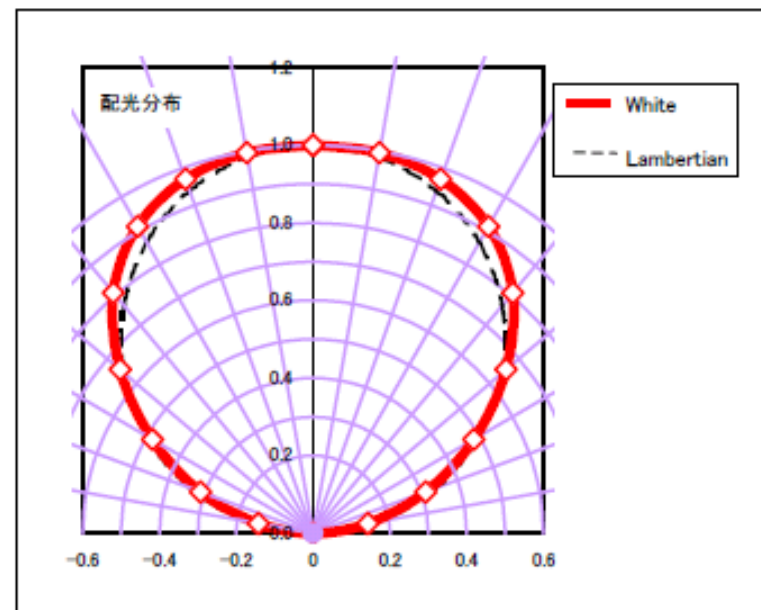
Light Distribution Curve
